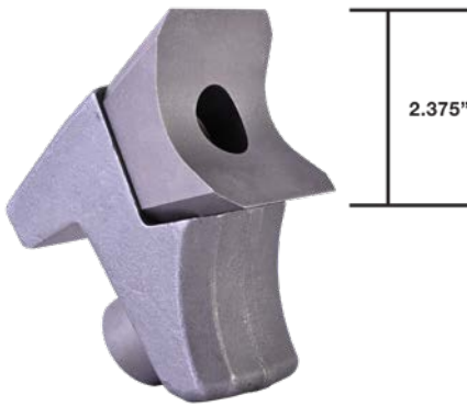
T9000 BOLT-ON PLANER TIP TOOTH*
